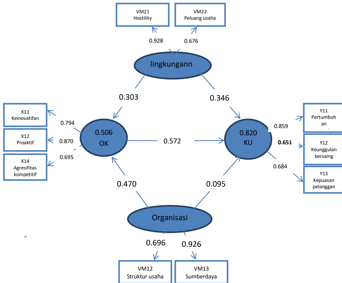
Gambar 1 Diagram path model resipikasi akhir loading factor
